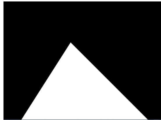
Figure 7: Masked Image
